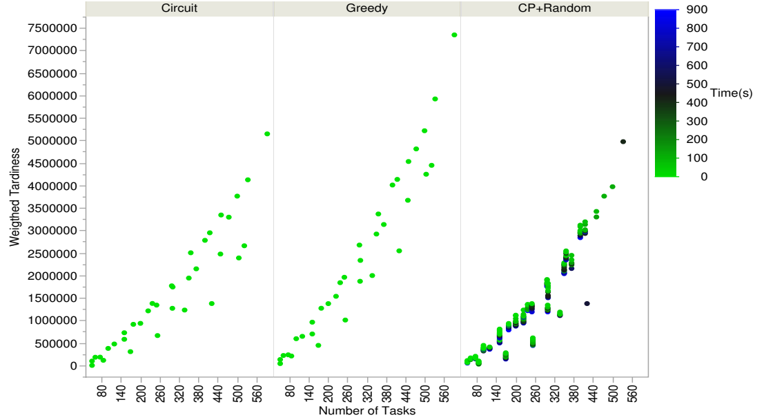
Fig. 3: Comparison between CIRCUI, GREEDY, and one of the methods based on CP
