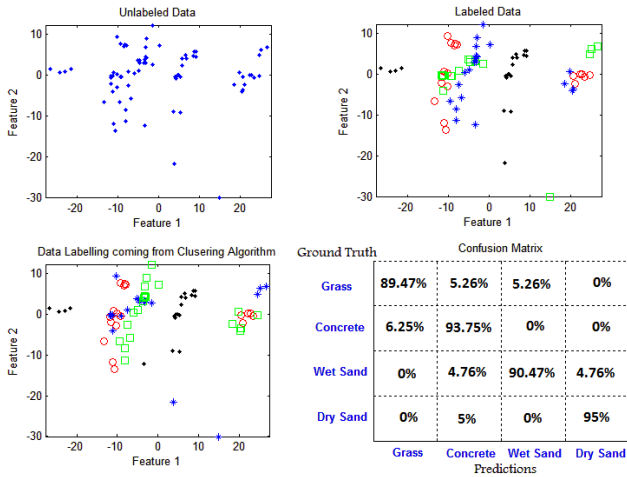
Figure 9. Results of the classification algorithm run on the data set collected at a speed ( C_f ) of 0.4 and N_f=5 (PCA features) selected from the data. Also shows the confusion matrix of the classification.
